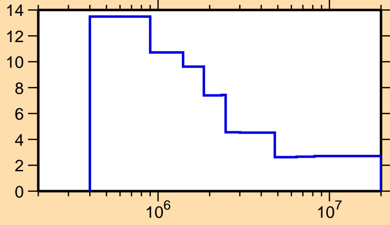
\Delta\sigma/\sigma vs. E for ^{167}\text{Yb}(n,n\text{onel.})
