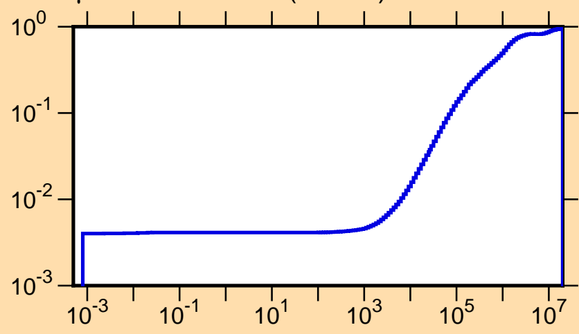
\mu vs. E for ^{168}\text{Yb}(\text{mt251})
