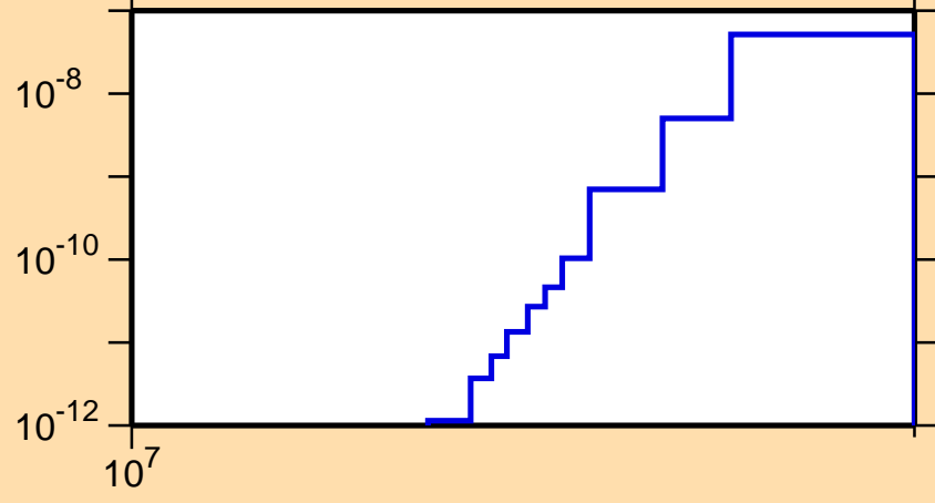
\sigma vs. E for ^{168}\text{Yb}(n,\text{He3})
