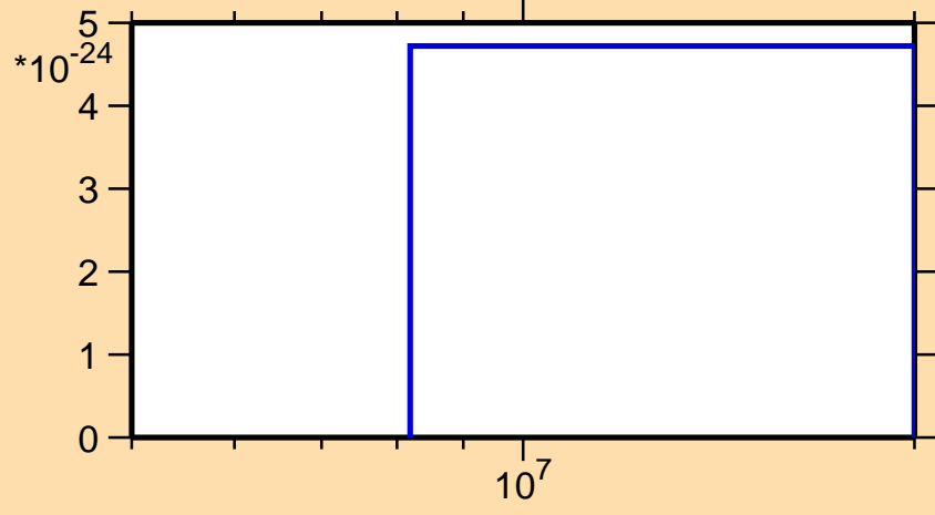
\sigma vs. E for ^{168}\text{Yb} (mt 11)
