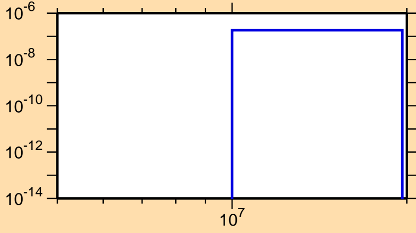
\sigma vs. E for ^{169}\text{Yb}(n,2n\alpha)
