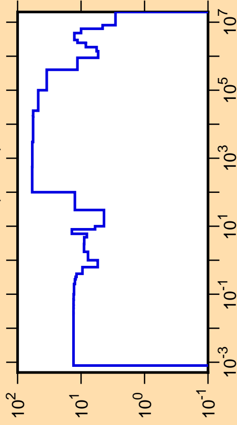
\Delta\sigma/\sigma vs. E for ^{169}\text{Yb}(n,\text{tot.})
