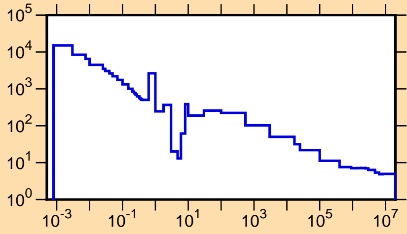
\sigma vs. E for ^{169}\text{Yb}(n,\text{tot.})
