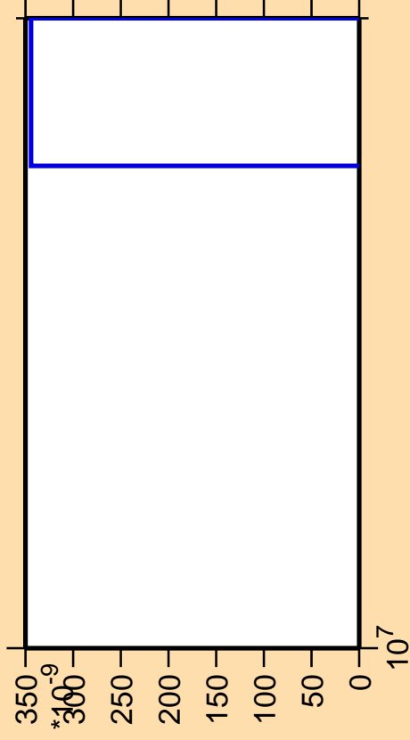
\Delta\sigma/\sigma vs. E for ^{169}\text{Yb} (mt 11)
