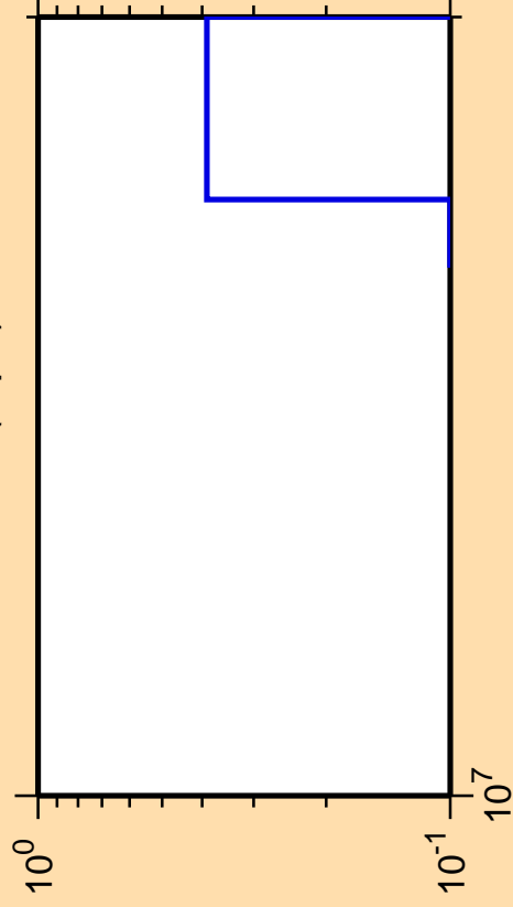
\Delta\sigma/\sigma vs. E for ^{169}\text{Yb}(n,\text{pd})
