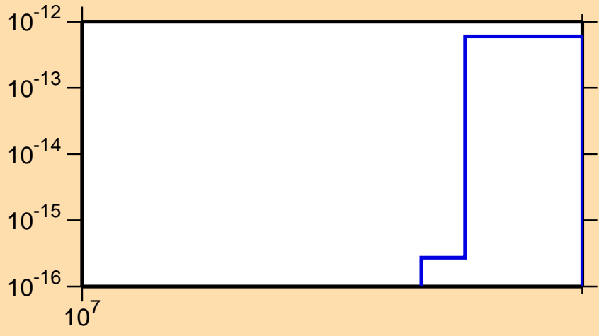
\sigma vs. E for ^{169}\text{Yb} (mt 34)
