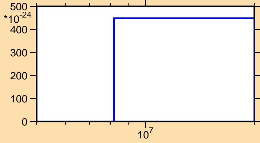
\sigma vs. E for ^{169}\text{Yb} (mt 11)
