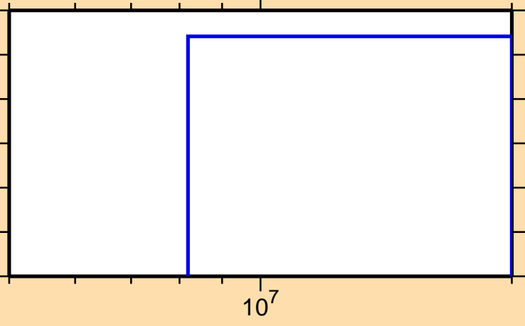
\sigma vs. E for ^{169}\text{Yb}(n,\text{He3})
