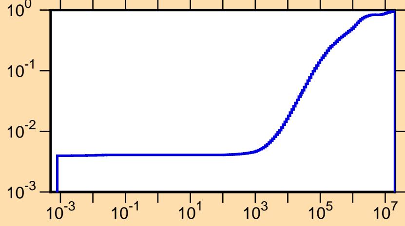
\mu vs. E for ^{170}\text{Yb}(\text{mt251})
