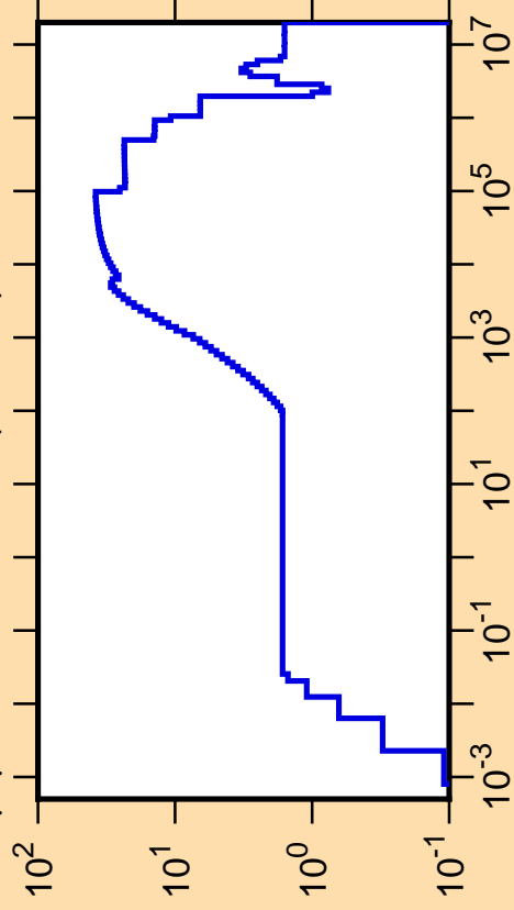
\Delta\mu/\mu vs. E for ^{170}\text{Yb}(\text{mt251})
