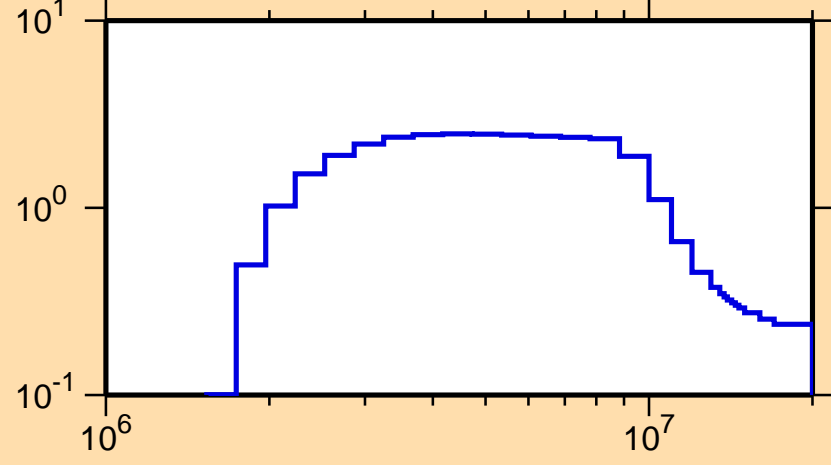
\sigma vs. E for ^{170}\text{Yb}(n,n\text{cont.})
