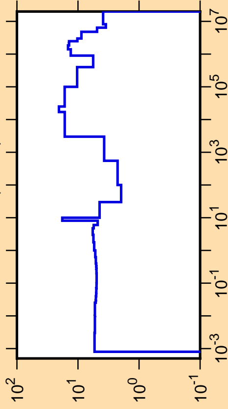
\Delta\sigma/\sigma vs. E for ^{171}\text{Yb}(n,\text{tot.})
