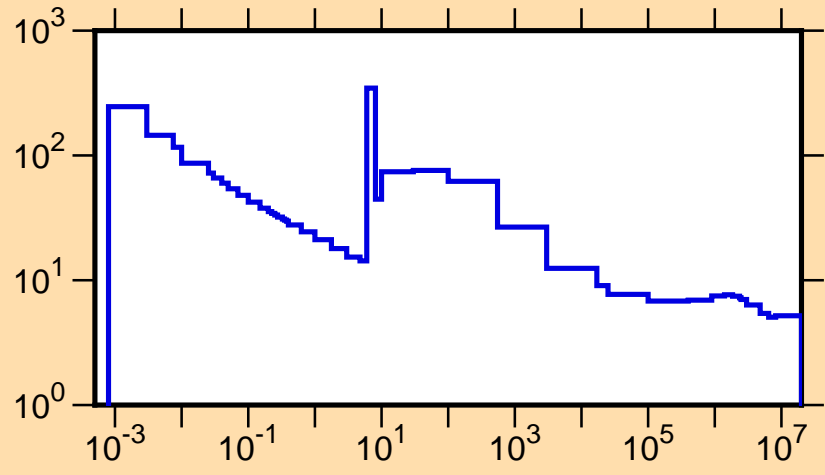
\sigma vs. E for ^{171}\text{Yb}(n,\text{tot.})
