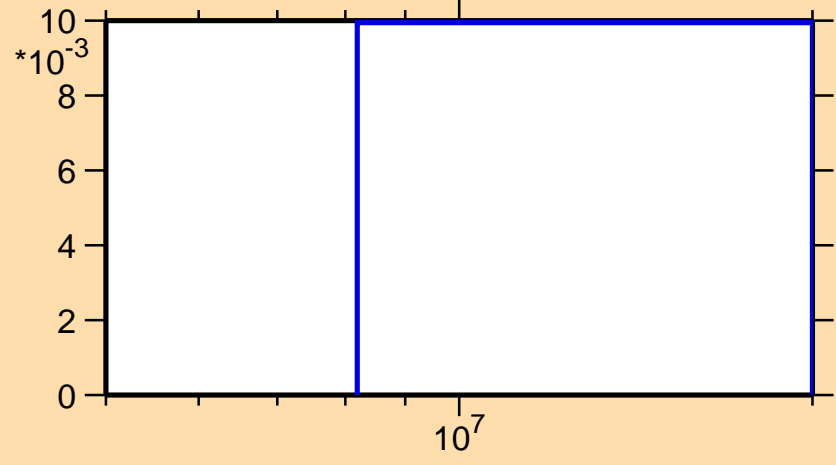
\sigma vs. E for ^{171}\text{Yb}(n,3n)
