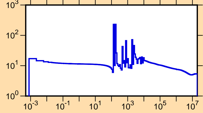
\sigma vs. E for ^{172}\text{Yb}(n,\text{tot.})
