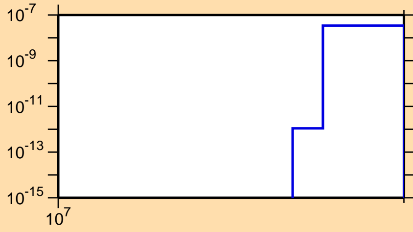
\sigma vs. E for ^{172}\text{Yb}(n,2np)
