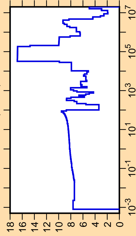
\Delta\sigma/\sigma vs. E for ^{172}\text{Yb}(n,\text{tot.})
