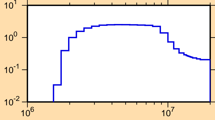
\sigma vs. E for ^{172}\text{Yb}(n,n\text{cont.})
