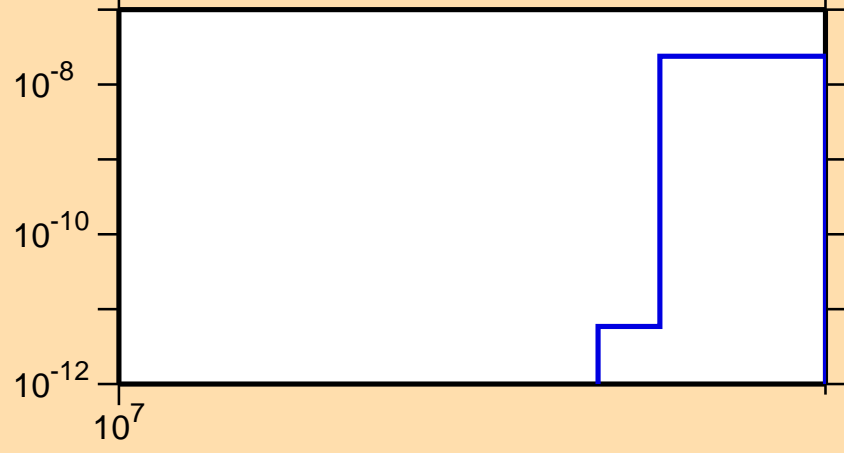
\sigma vs. E for ^{172}\text{Yb}(n,nt)
