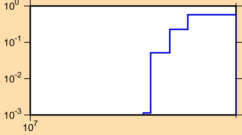
\sigma vs. E for ^{172}\text{Yb}(n,3n)
