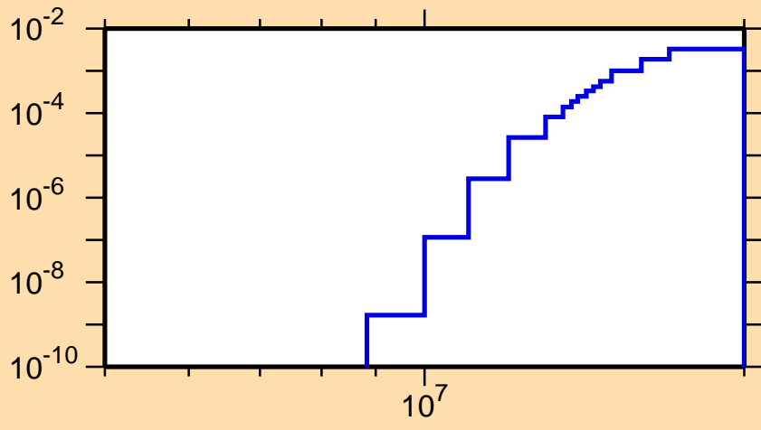
\sigma vs. E for ^{172}\text{Yb}(n,d)
