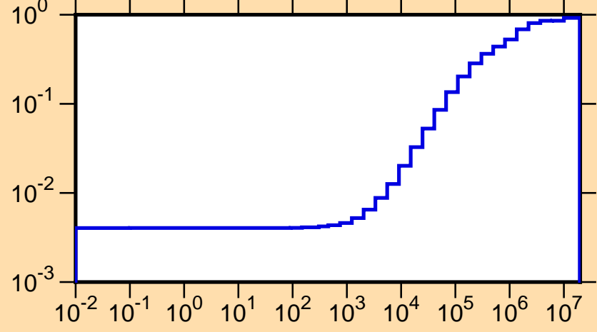
\mu vs. E for ^{172}\text{Yb}(\text{mt251})
