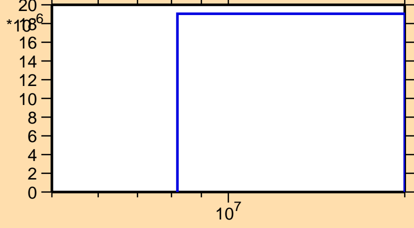
\sigma vs. E for ^{172}\text{Yb}(n,t)
