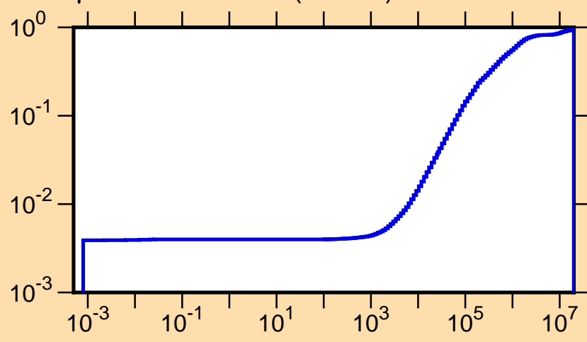
\mu vs. E for ^{173}\text{Yb}(\text{mt251})
