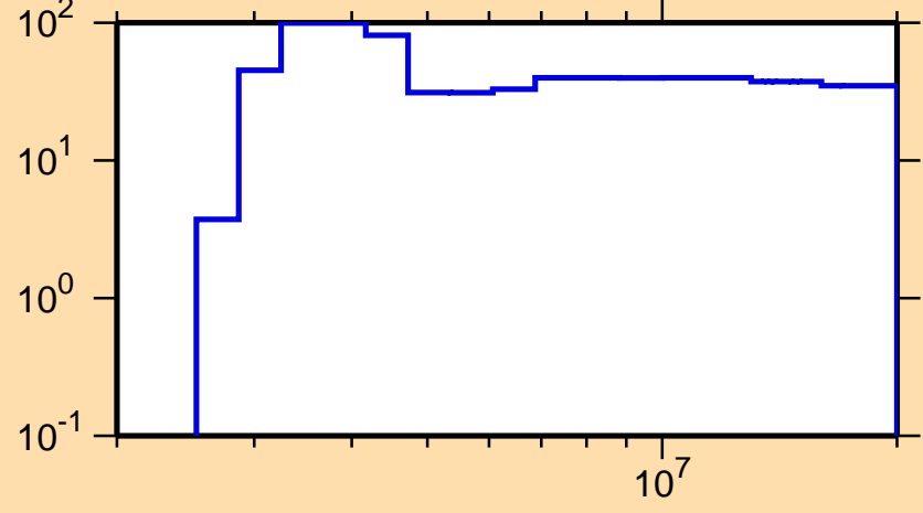
\Delta\sigma/\sigma vs. E for ^{173}\text{Yb}(n,p)
