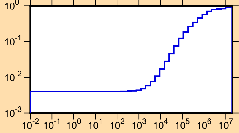
\mu vs. E for ^{173}\text{Yb}(\text{mt251})
