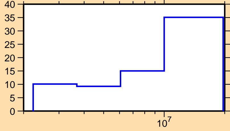
\Delta\sigma/\sigma vs. E for ^{173}\text{Yb}(n,ncont.)
