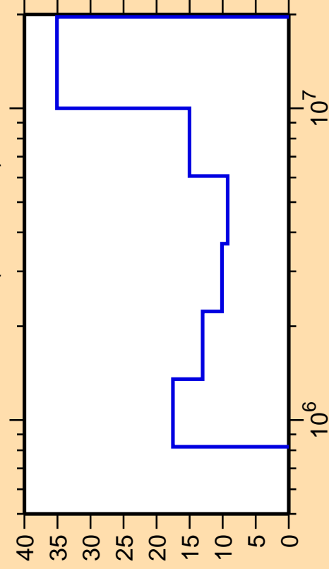
\Delta\sigma/\sigma vs. E for ^{173}\text{Yb}(n,\text{ncont.})
