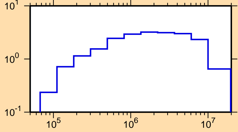
\sigma vs. E for ^{173}\text{Yb}(n,\text{inel.})
