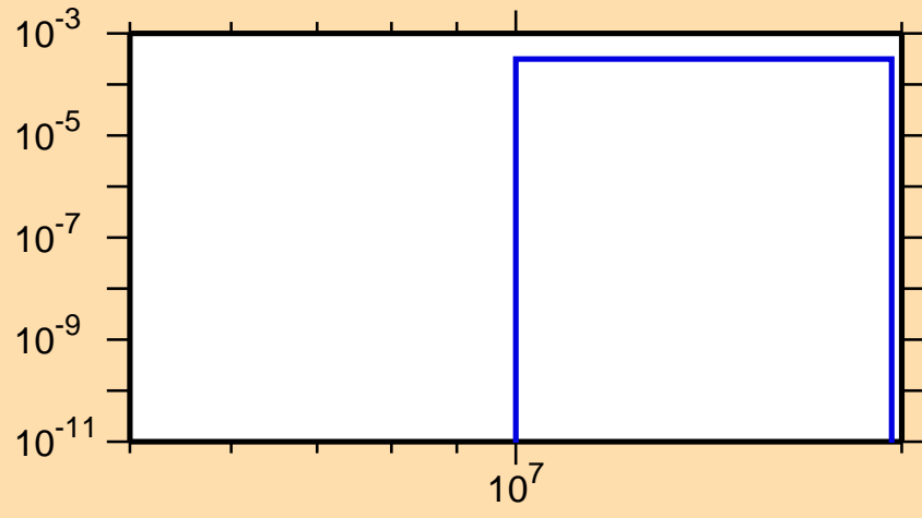
\sigma vs. E for ^{173}\text{Yb}(n,np)
