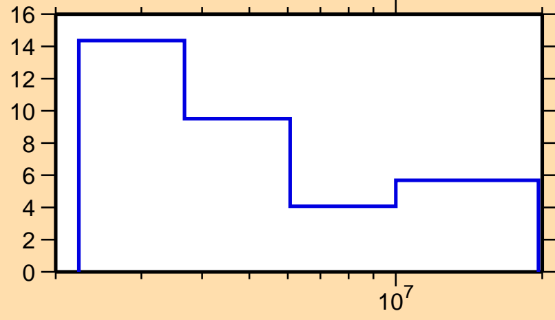
\Delta\sigma/\sigma vs. E for ^{173}\text{Yb}(n,el.)
