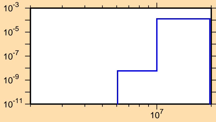
\sigma vs. E for ^{173}\text{Yb}(n,n\alpha)
