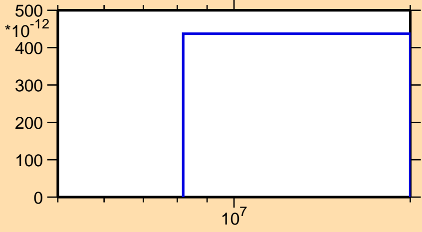
\sigma vs. E for ^{173}\text{Yb}(n,\text{nt})
