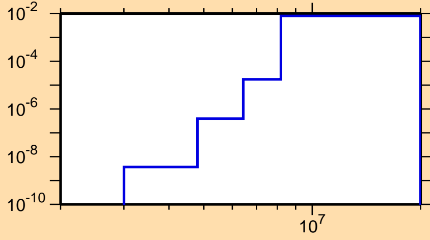
\sigma vs. E for ^{173}\text{Yb}(n,p)
