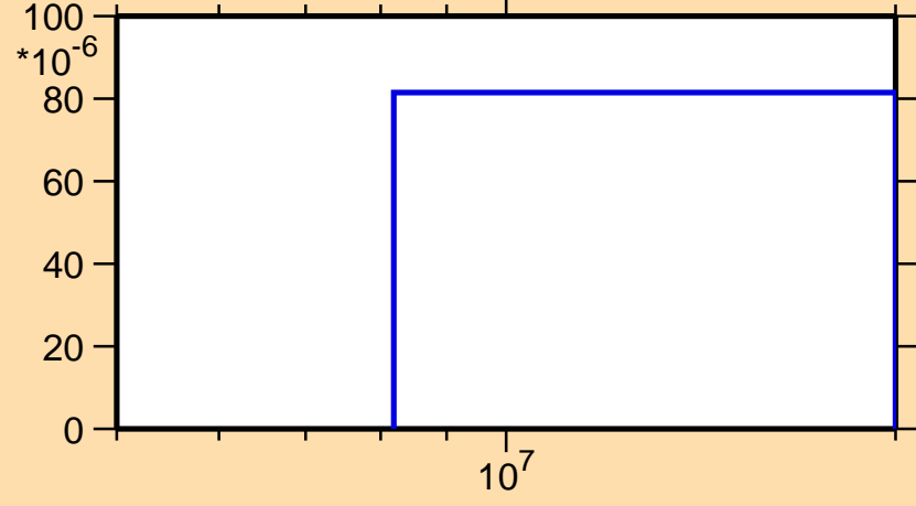
\sigma vs. E for ^{173}\text{Yb}(n,t)
