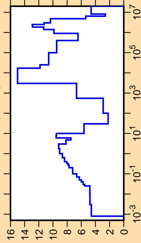
\Delta\sigma/\sigma vs. E for ^{173}\text{Yb}(n,\text{tot.})
