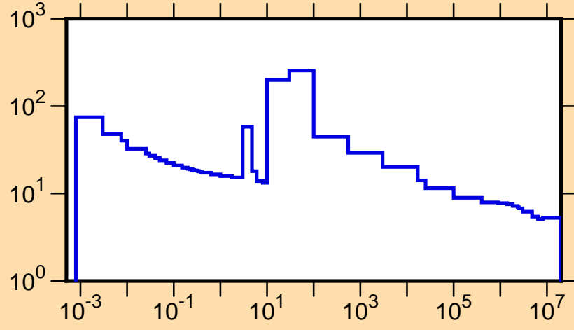
\sigma vs. E for ^{173}\text{Yb}(n,\text{tot.})
