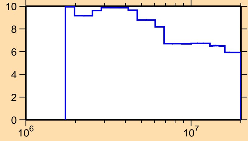
\Delta\sigma/\sigma vs. E for ^{174}\text{Yb}(n,n\text{inel.})
