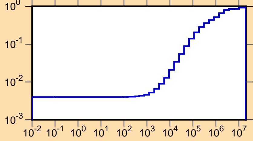
\mu vs. E for ^{174}\text{Yb}(\text{mt251})
