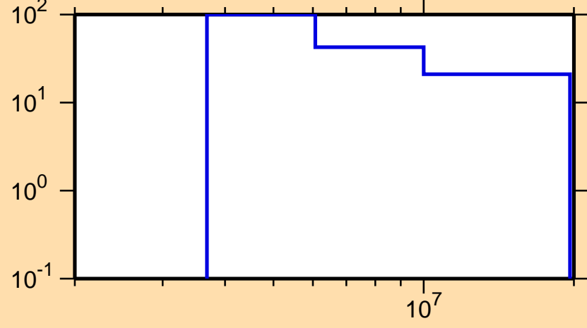
\Delta\sigma/\sigma vs. E for ^{174}\text{Yb}(n,p)
