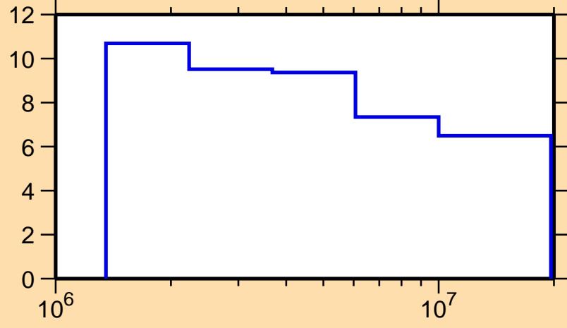
\Delta\sigma/\sigma vs. E for ^{174}\text{Yb}(n,n\text{nonel.})
