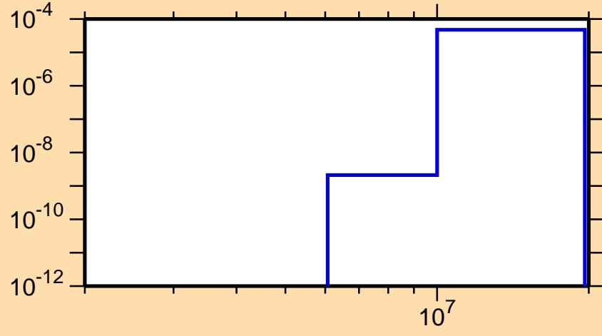
\sigma vs. E for ^{174}\text{Yb}(n,n\alpha)
