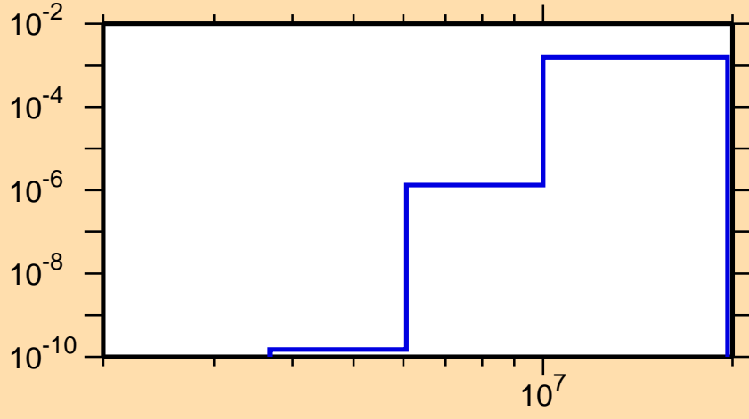
\sigma vs. E for ^{174}\text{Yb}(n,p)
