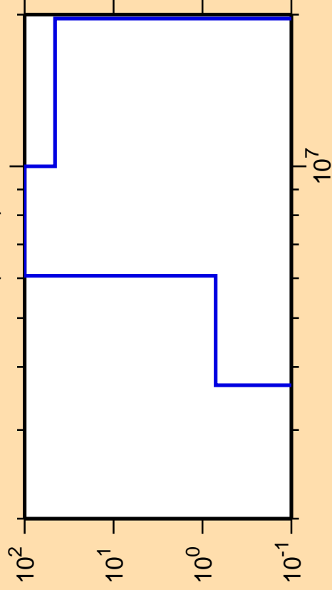
\Delta\sigma/\sigma vs. E for ^{174}\text{Yb}(n,n\alpha)
