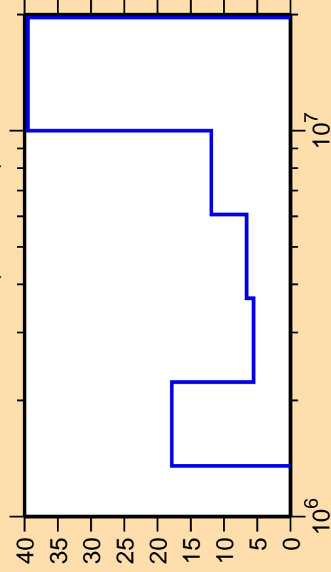
\Delta\sigma/\sigma vs. E for ^{174}\text{Yb}(n,\text{ncont.})
