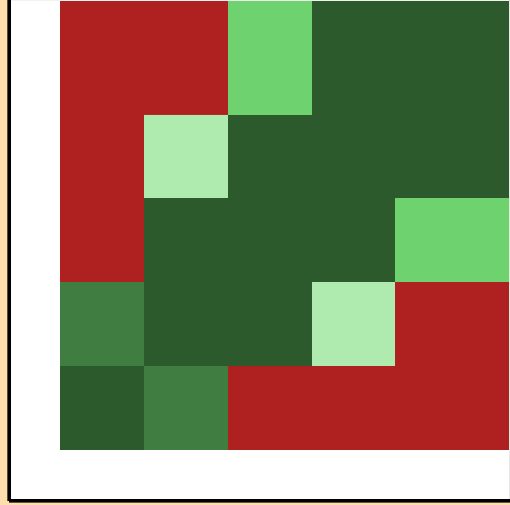
\sigma vs. E for ^{174}\text{Yb}(n,n\text{cont.})
