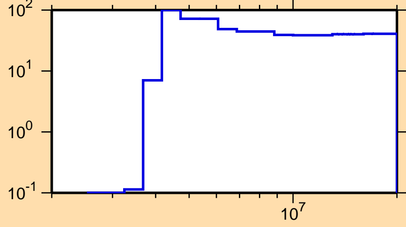
\Delta\sigma/\sigma vs. E for ^{175}\text{Yb}(n,p)
