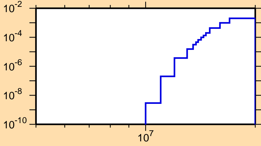
\sigma vs. E for ^{175}\text{Yb}(n,d)
