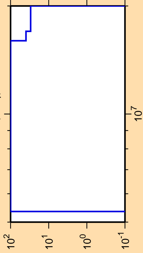
\Delta\sigma/\sigma vs. E for ^{175}\text{Yb}(n,n_1)
