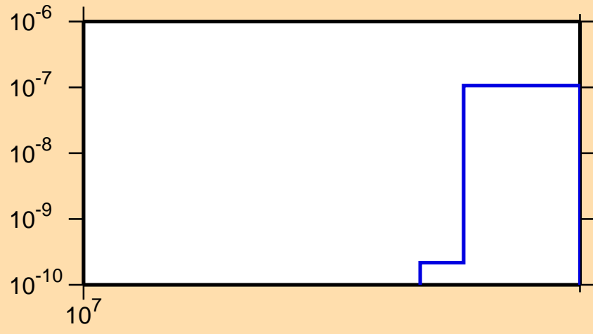
\sigma vs. E for ^{175}\text{Yb}(n,nt)
