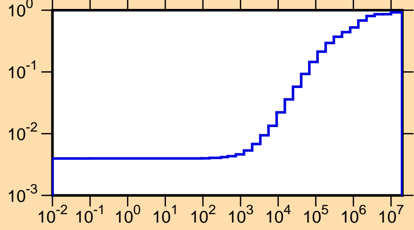
\mu vs. E for ^{176}\text{Yb}(\text{mt251})
