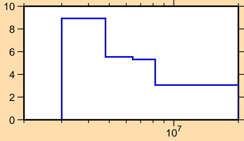
\Delta\sigma/\sigma vs. E for ^{176}\text{Yb}(n,el.)
