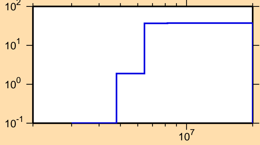
\Delta\sigma/\sigma vs. E for ^{176}\text{Yb}(n,p)
