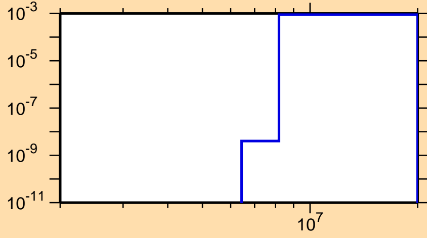
\sigma vs. E for ^{176}\text{Yb}(n,p)
