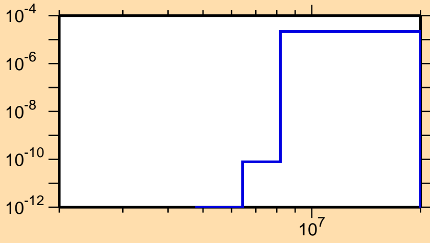
\sigma vs. E for ^{176}\text{Yb}(n,n\alpha)
