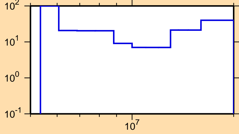
\Delta\sigma/\sigma vs. E for ^{176}\text{Yb}(n,2n)
