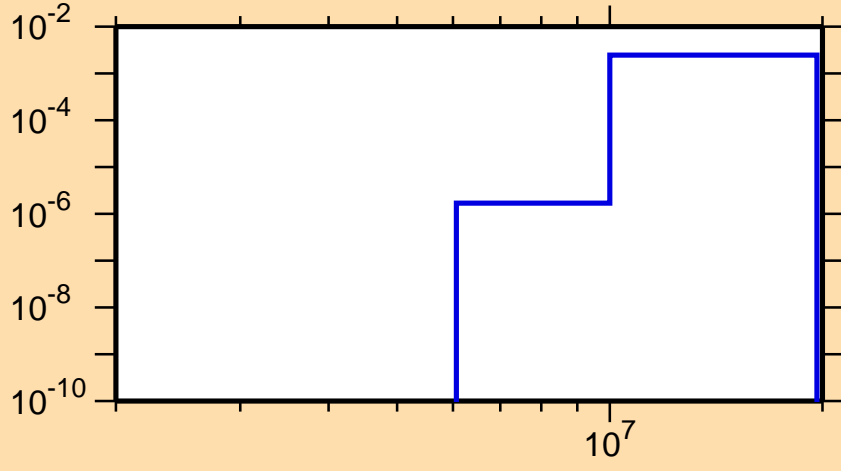
\sigma vs. E for ^{176}\text{Yb}(n,p)
