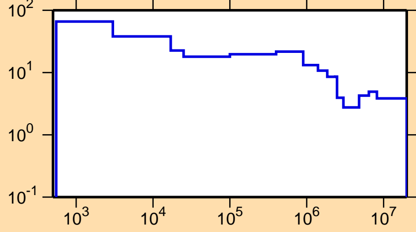
\Delta\sigma/\sigma vs. E for ^{176}\text{Yb}(n,\text{nonel.})
