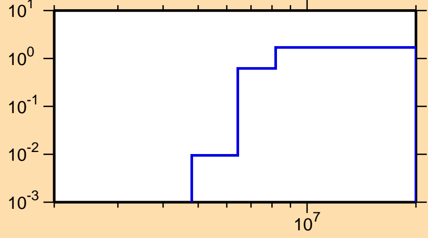
\sigma vs. E for ^{176}\text{Yb}(n,2n)
