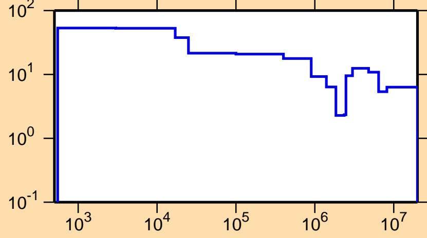
\Delta\sigma/\sigma vs. E for ^{176}\text{Yb}(n,\text{el.})
