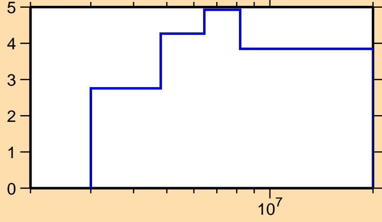
\Delta\sigma/\sigma vs. E for ^{176}\text{Yb}(n,\text{nonel.})
