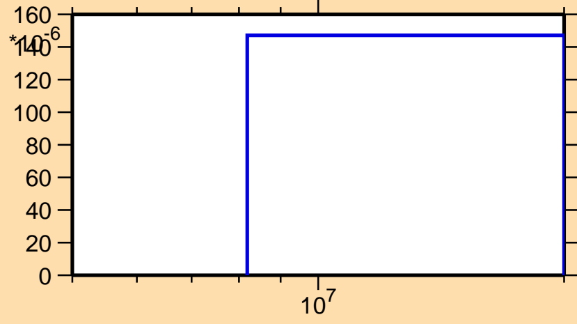
\sigma vs. E for ^{176}\text{Yb}(n,d)
