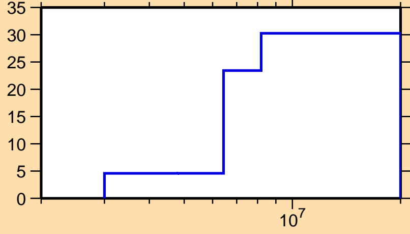
\Delta\sigma/\sigma vs. E for ^{176}\text{Yb}(n,ncont.)
