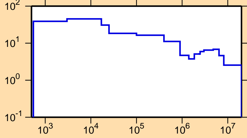
\Delta\sigma/\sigma vs. E for ^{176}\text{Yb}(n,\text{tot.})
