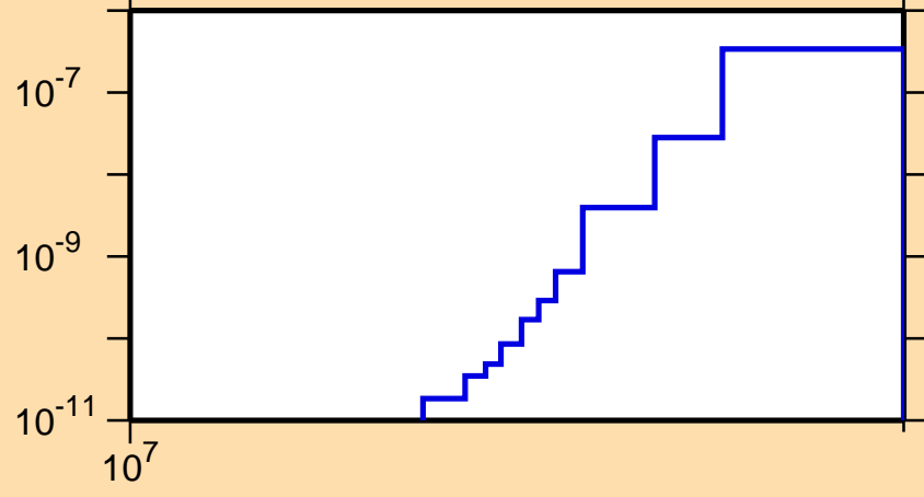
\sigma vs. E for ^{177}\text{Yb}(n,2n\alpha)
