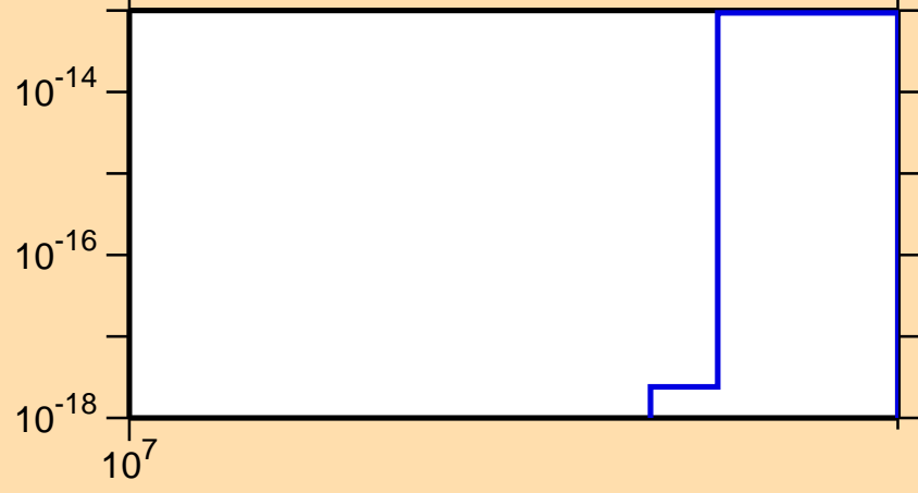
\sigma vs. E for ^{177}\text{Yb}(n,\text{He3})
