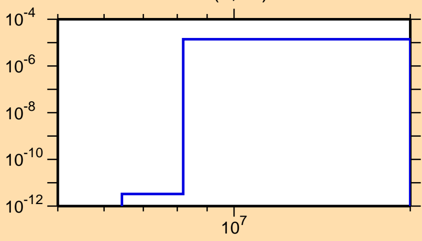
\sigma vs. E for ^{177}\text{Yb}(n,n\alpha)
