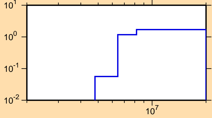
\sigma vs. E for ^{177}\text{Yb}(n,2n)
