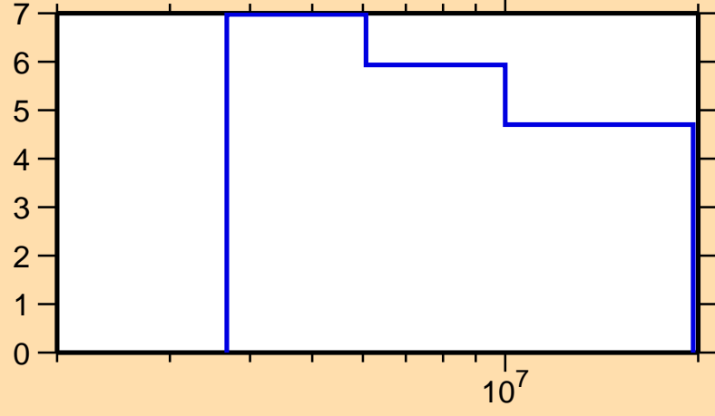
\Delta\sigma/\sigma vs. E for ^{177}\text{Yb}(n,\text{nonel.})
