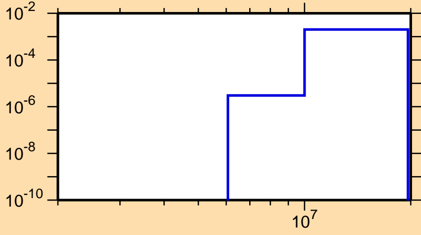
\sigma vs. E for ^{177}\text{Yb}(n,p)
