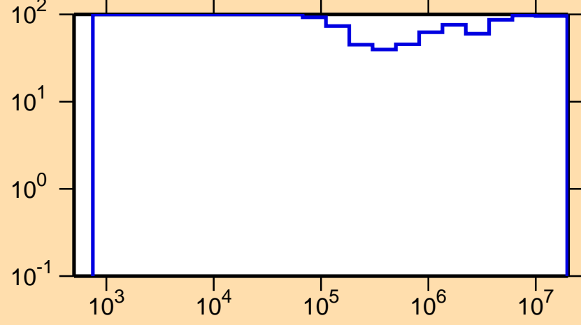
\Delta\sigma/\sigma vs. E for ^{177}\text{Yb}(n,n_1)
