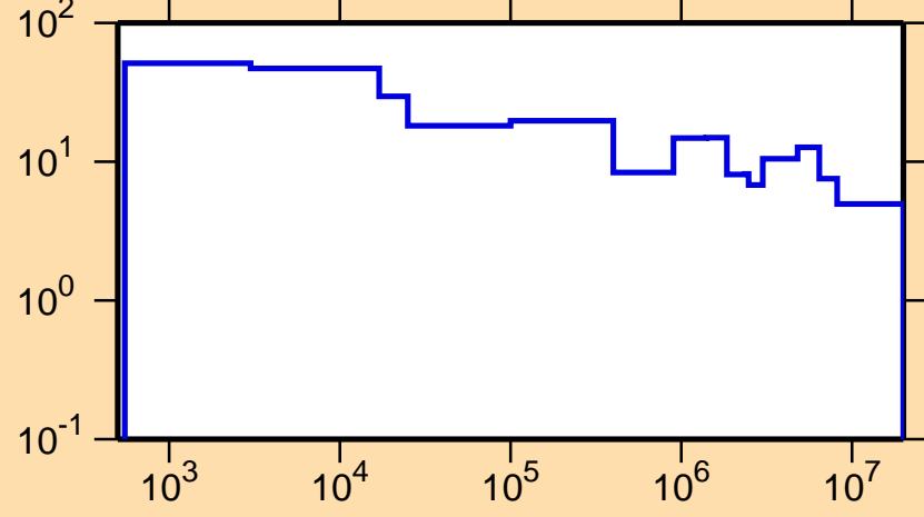
\Delta\sigma/\sigma vs. E for ^{177}\text{Yb}(n,\text{el.})
