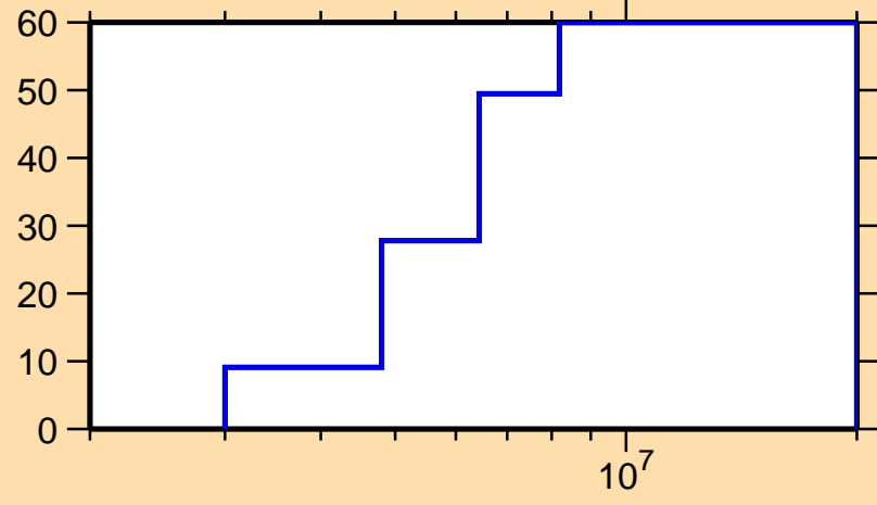
\Delta\sigma/\sigma vs. E for ^{177}\text{Yb}(n,ncont.)
