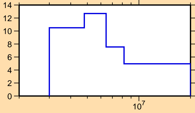
\Delta\sigma/\sigma vs. E for ^{177}\text{Yb}(n,el.)
