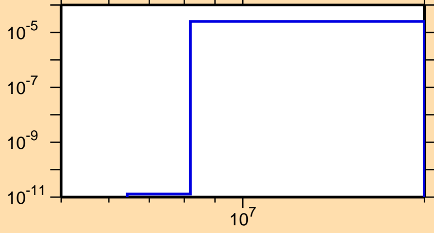
\sigma vs. E for ^{177}\text{Yb}(n,n\alpha)
