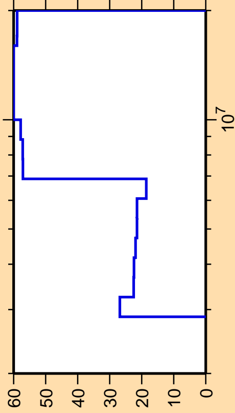
\Delta\sigma/\sigma vs. E for ^{178}\text{Yb}(n,\text{ncont.})
