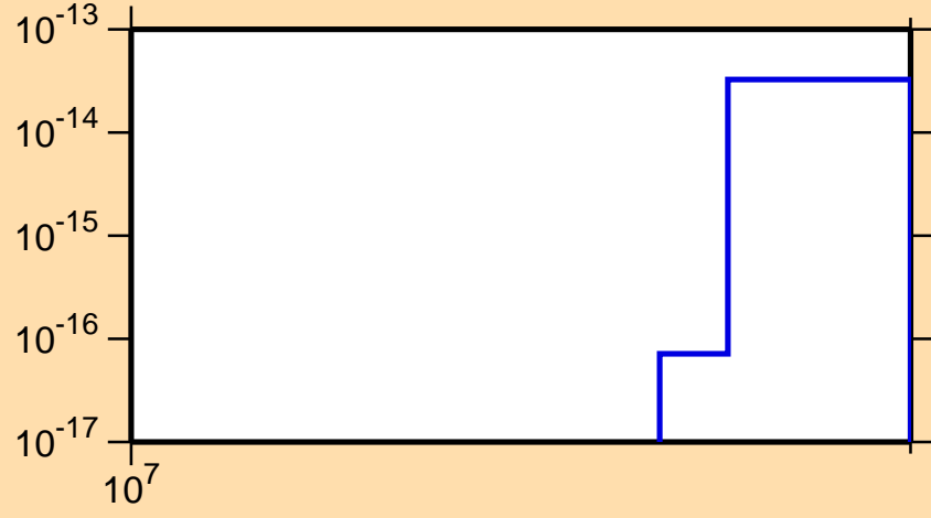
\sigma vs. E for ^{178}\text{Yb}(n,3n\alpha)
