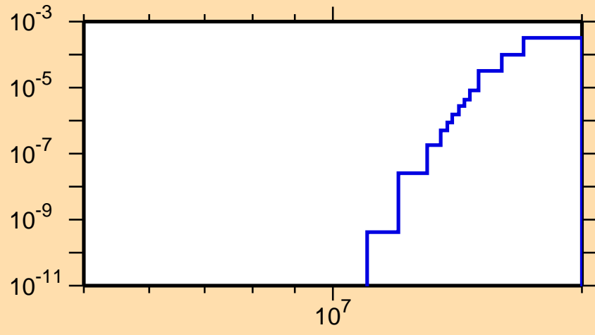
\sigma vs. E for ^{178}\text{Yb}(n,d)
