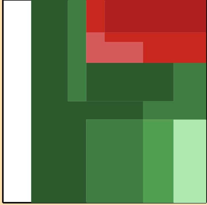
\Delta\sigma/\sigma vs. E for ^{178}\text{Yb}(n,p)
