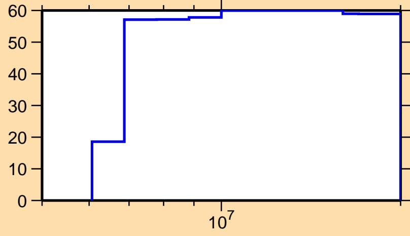
\Delta\sigma/\sigma vs. E for ^{178}\text{Yb}(n,ncont.)
