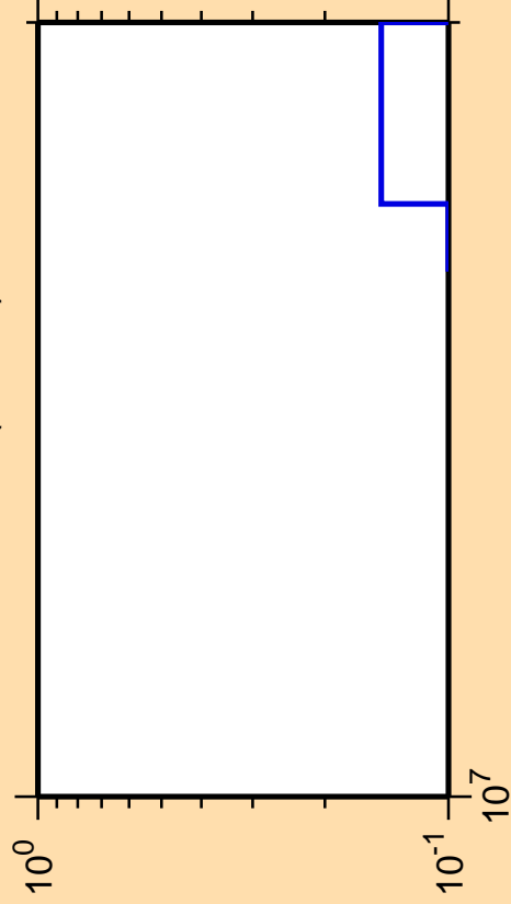
\Delta\sigma/\sigma vs. E for ^{178}\text{Yb}(n,3n\alpha)
