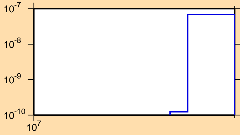
\sigma vs. E for ^{178}\text{Yb}(n,nt)
