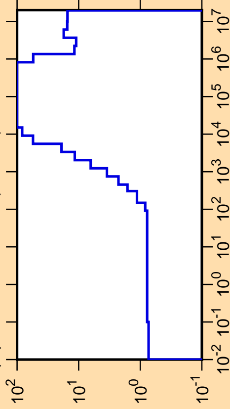
\Delta\mu/\mu vs. E for ^{178}\text{Yb}(\text{mt251})
