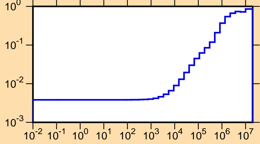
\mu vs. E for ^{178}\text{Yb}(\text{mt251})
