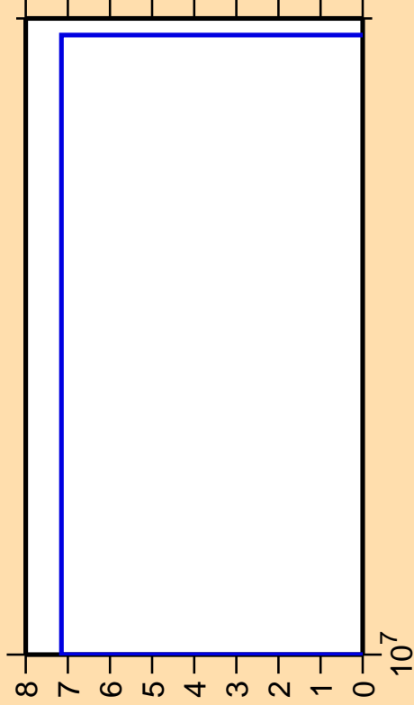
\Delta\sigma/\sigma vs. E for ^{178}\text{Yb}(n,2np)
