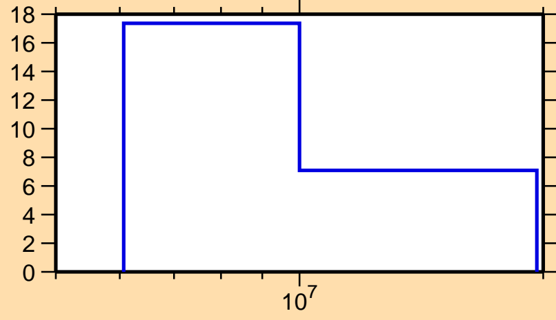
\Delta\sigma/\sigma vs. E for ^{178}\text{Yb}(n,el.)
