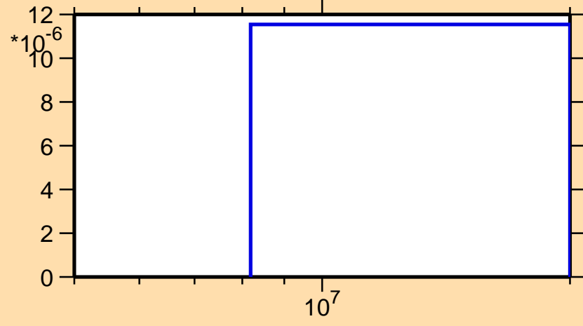
\sigma vs. E for ^{178}\text{Yb}(n,d)
