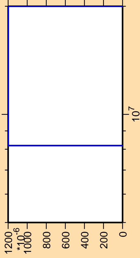
\Delta\sigma/\sigma vs. E for ^{178}\text{Yb}(n,3n\alpha)
