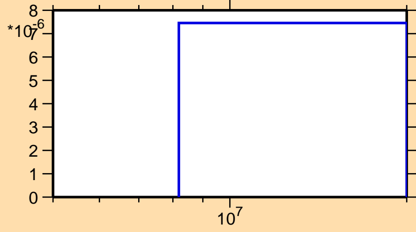
\sigma vs. E for ^{178}\text{Yb}(n,np)
