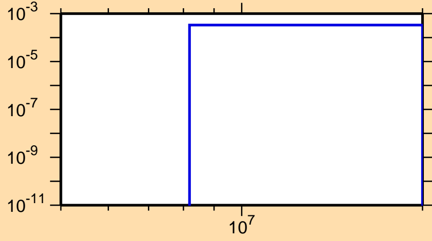
\sigma vs. E for ^{178}\text{Yb}(n,p)
