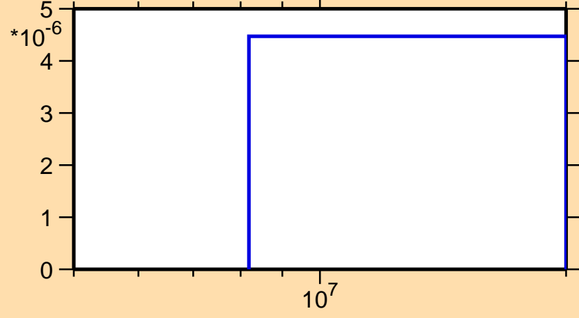
\sigma vs. E for ^{178}\text{Yb}(n,t)
