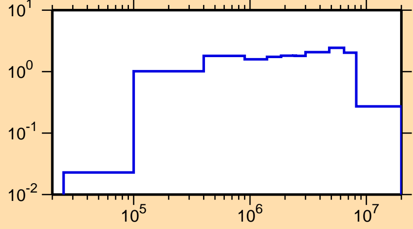
\sigma vs. E for ^{178}\text{Yb}(n,\text{inel.})
