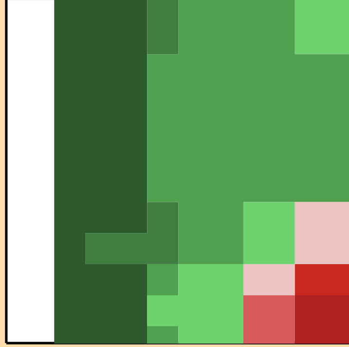
\Delta\sigma/\sigma vs. E for ^{179}\text{Yb}(n,p)
