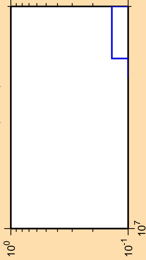
\Delta\sigma/\sigma vs. E for ^{179}\text{Yb}(n,3n\alpha)
