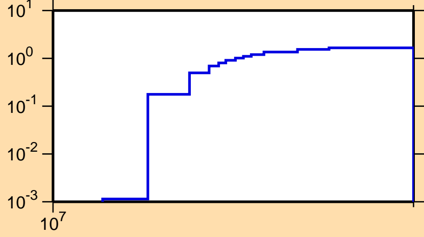
\sigma vs. E for ^{179}\text{Yb}(n,3n)
