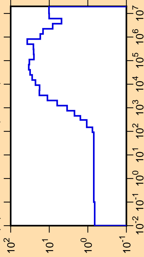
\Delta\mu/\mu vs. E for ^{179}\text{Yb}(\text{mt251})
