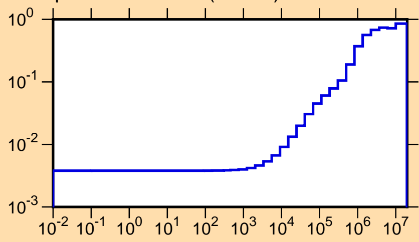
\mu vs. E for ^{179}\text{Yb}(\text{mt251})
