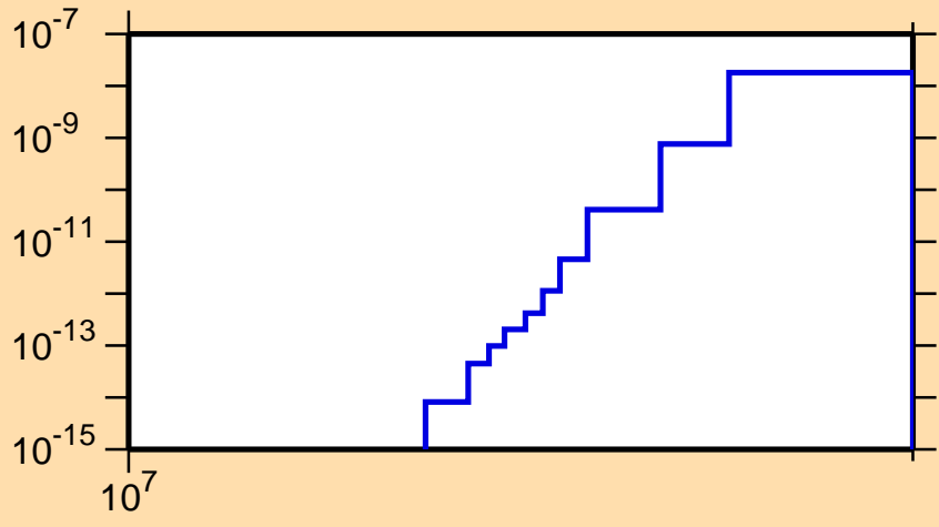
\sigma vs. E for ^{180}\text{Yb}(n,2n\alpha)
