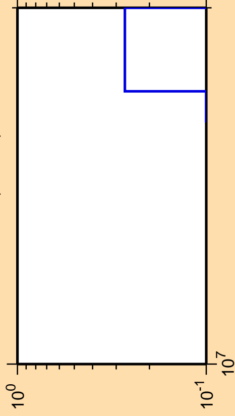
\Delta\sigma/\sigma vs. E for ^{180}\text{Yb}(n,3n\alpha)
