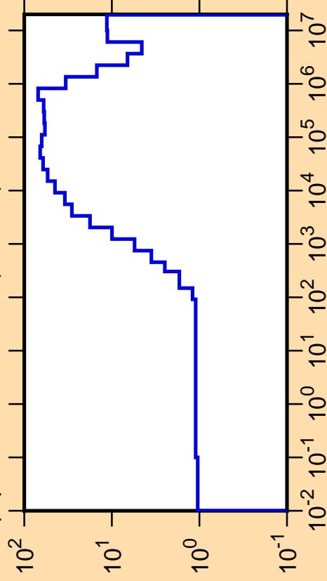
\Delta\mu/\mu vs. E for ^{181}\text{Yb}(\text{mt251})
