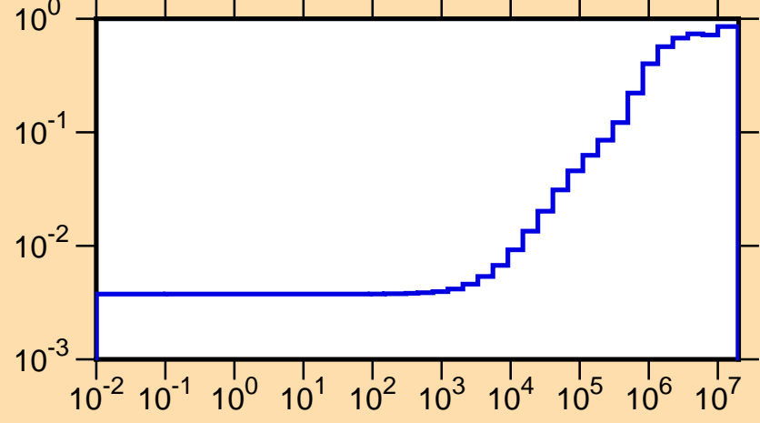
\mu vs. E for ^{181}\text{Yb}(\text{mt251})
