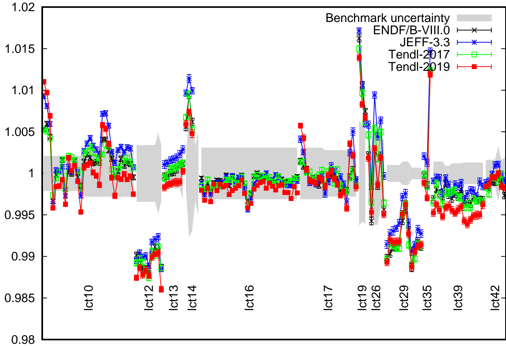
leu-comp-therm (2)
