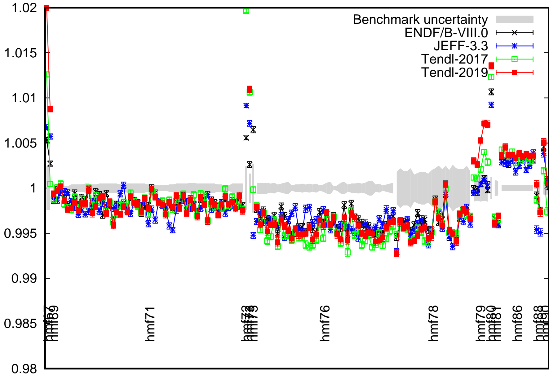
heu-met-fast (2)
