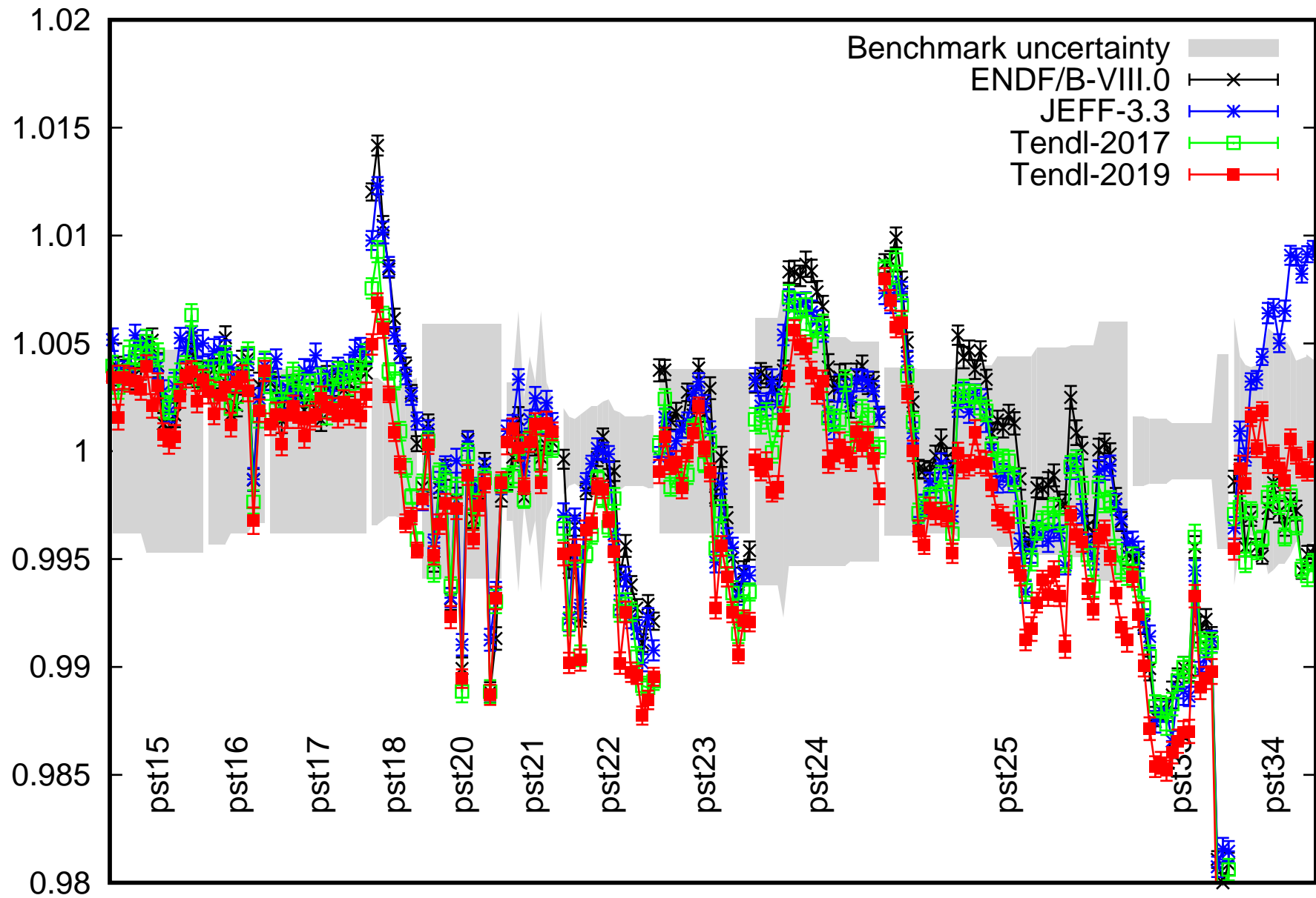
pu-sol-therm (2)
