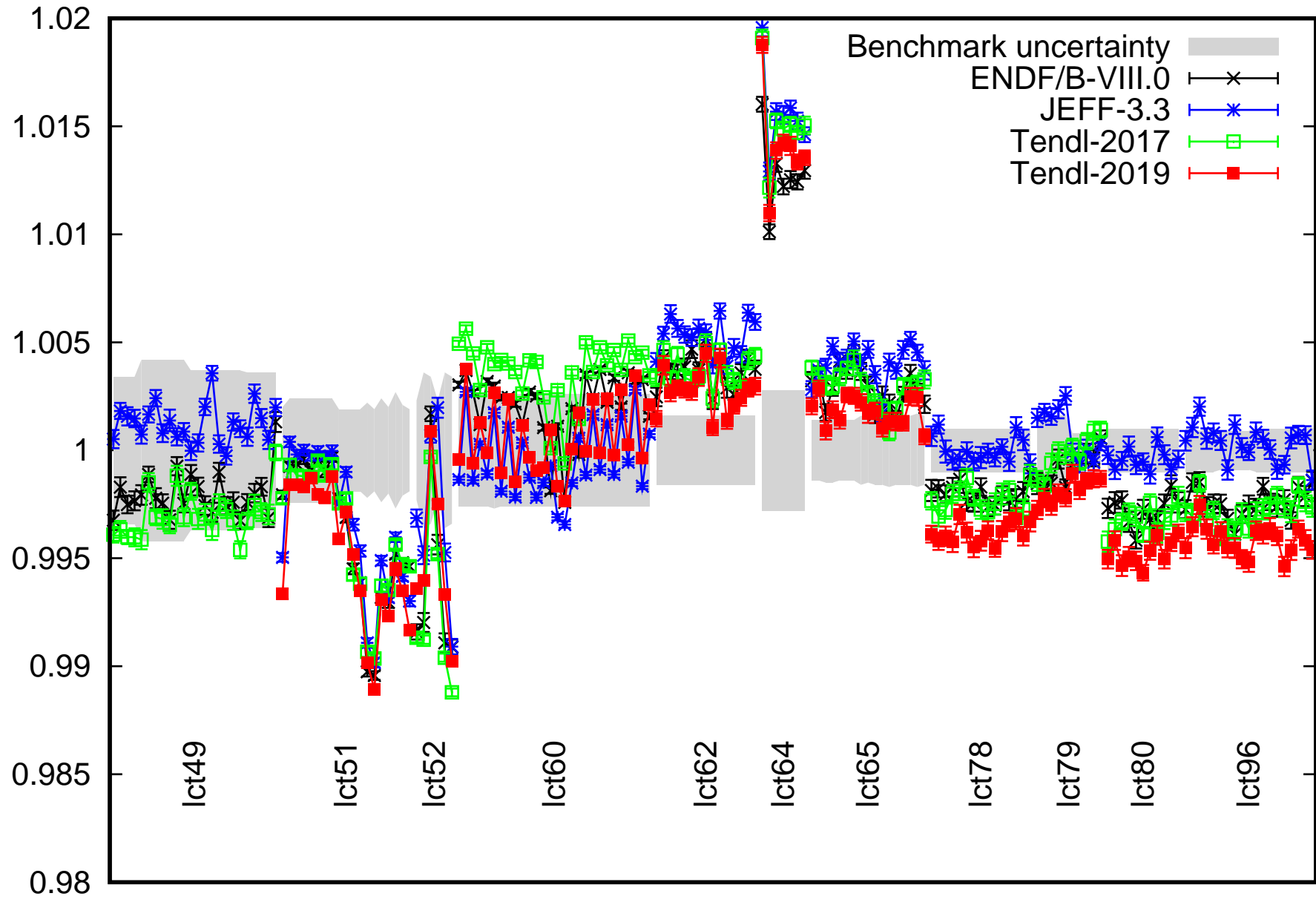
leu-comp-therm (3)
