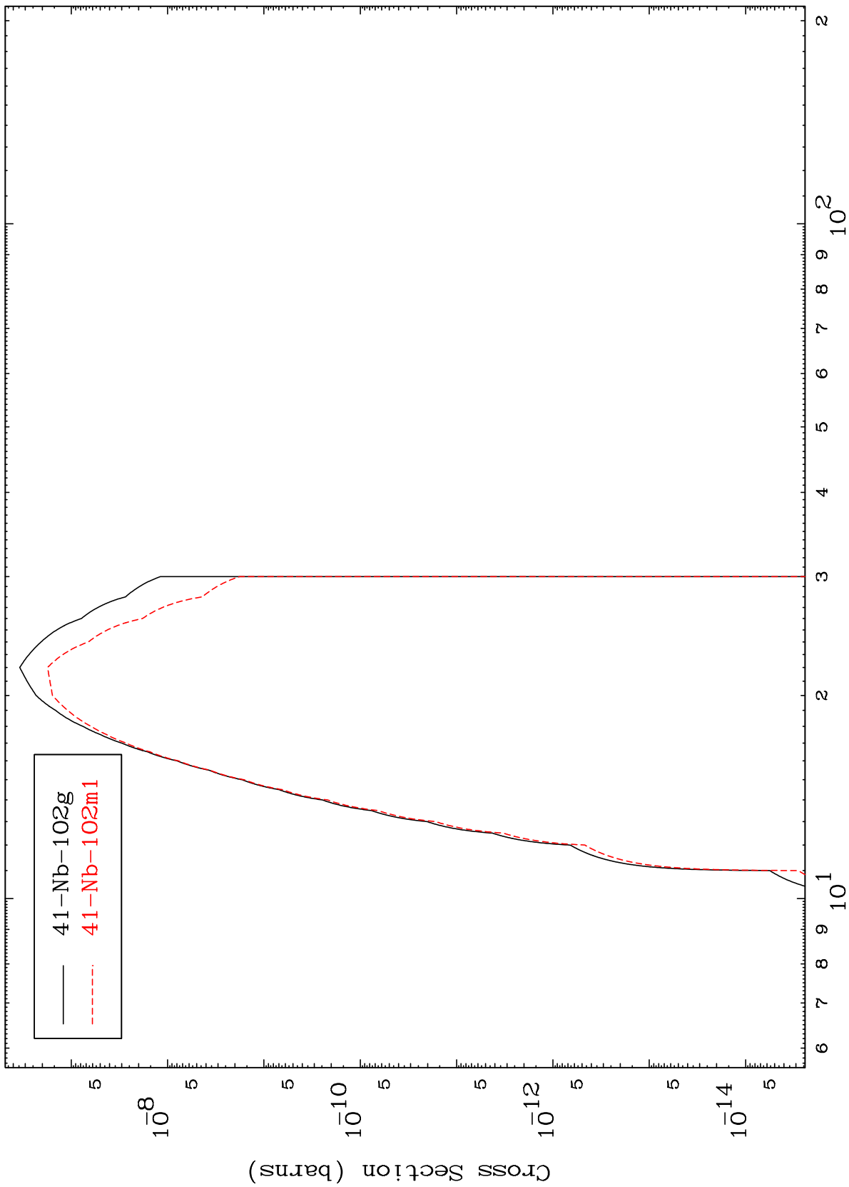
Radionuclide Production Cross Section ( \gamma, \alpha )
