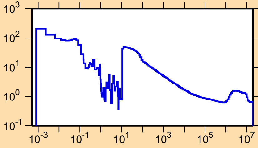
\sigma vs. E for ^{214}\text{Ac}(n,\text{nonel.})
