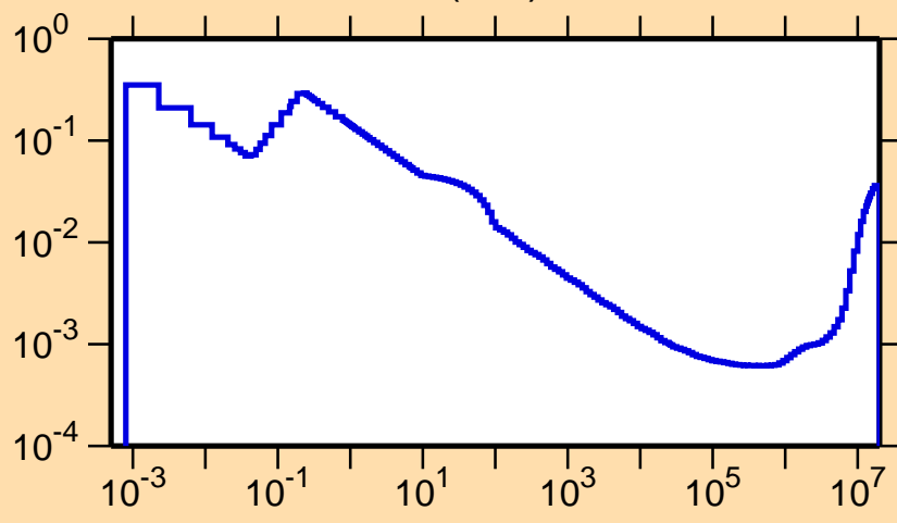
\sigma vs. E for ^{214}\text{Ac}(n,\alpha)
