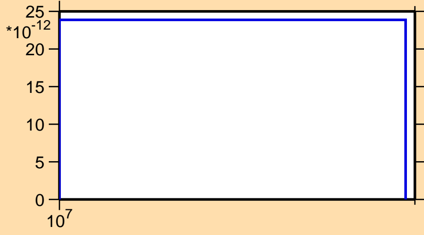
\sigma vs. E for ^{214}\text{Ac} (mt 34)
