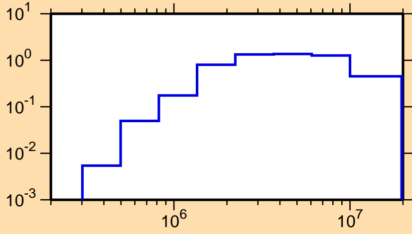
\sigma vs. E for ^{214}\text{Ac}(n,\text{inel.})
