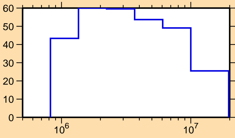
\Delta\sigma/\sigma vs. E for ^{214}\text{Ac}(n,n_1)
