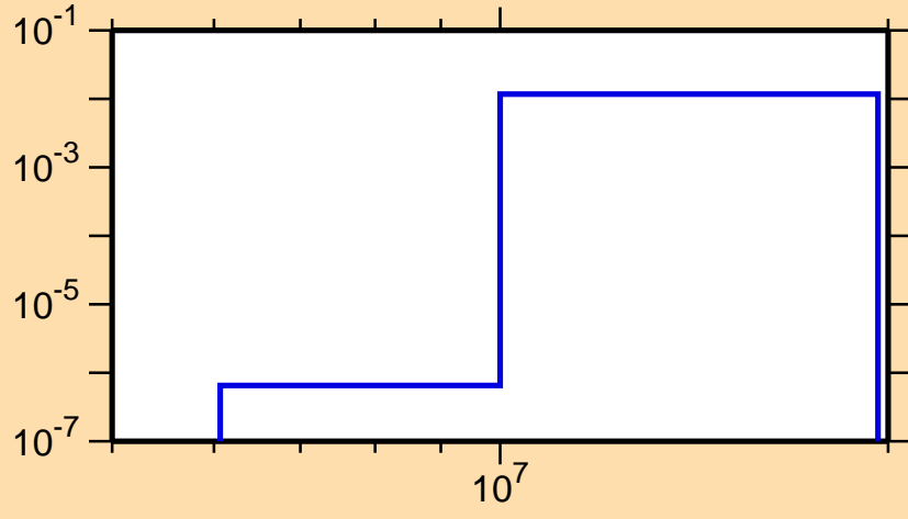
\sigma vs. E for ^{214}\text{Ac}(n,2n\alpha)
