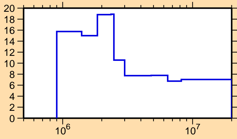
\Delta\sigma/\sigma vs. E for ^{214}\text{Ac}(n,\text{nonel.})
