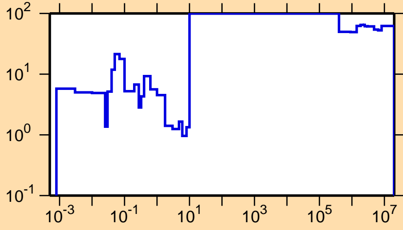
\Delta\sigma/\sigma vs. E for ^{214}\text{Ac}(n,\gamma)
