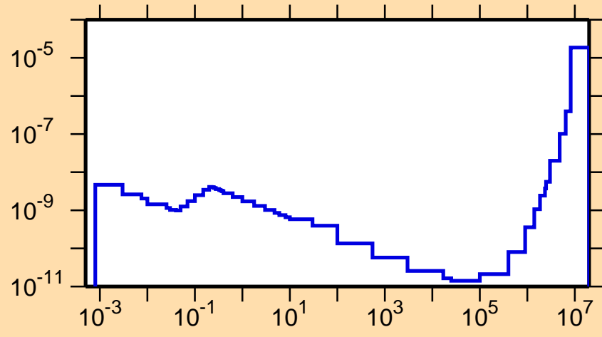
\sigma vs. E for ^{214}\text{Ac}(n,p\alpha)
