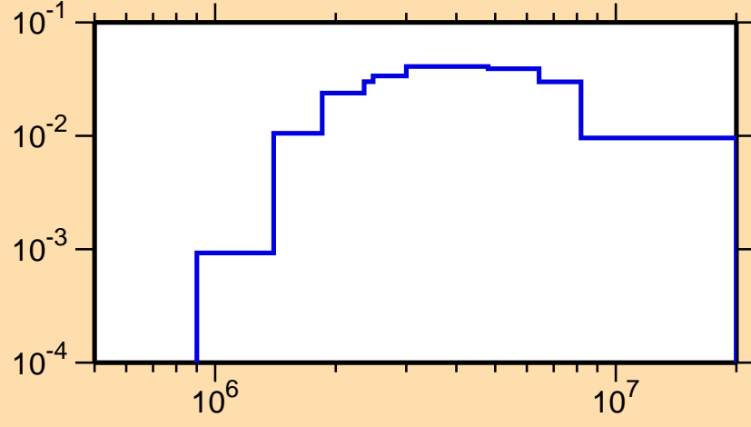
\sigma vs. E for ^{214}\text{Ac}(n,n\alpha)
