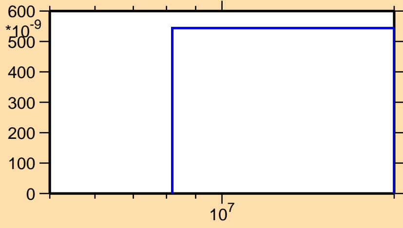
\sigma vs. E for ^{214}\text{Ac}(n,\text{nd})
