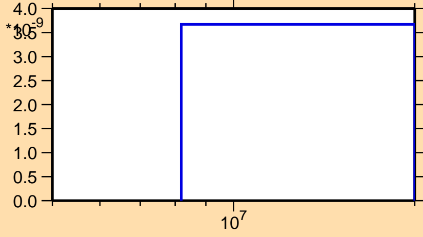
\sigma vs. E for ^{214}\text{Ac}(n,3n\alpha)
