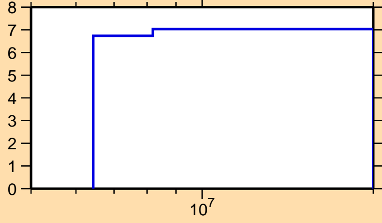
\Delta\sigma/\sigma vs. E for ^{214}\text{Ac}(n,\text{nonel.})
