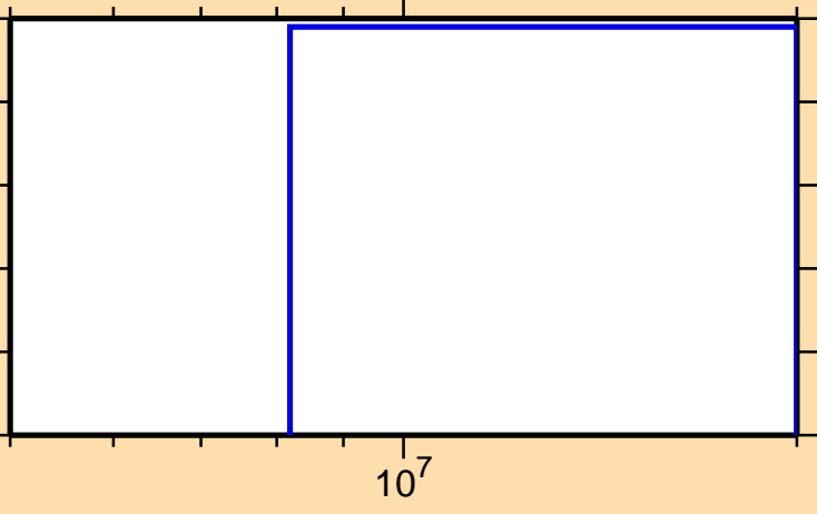
\sigma vs. E for ^{214}\text{Ac}(n,pd)
