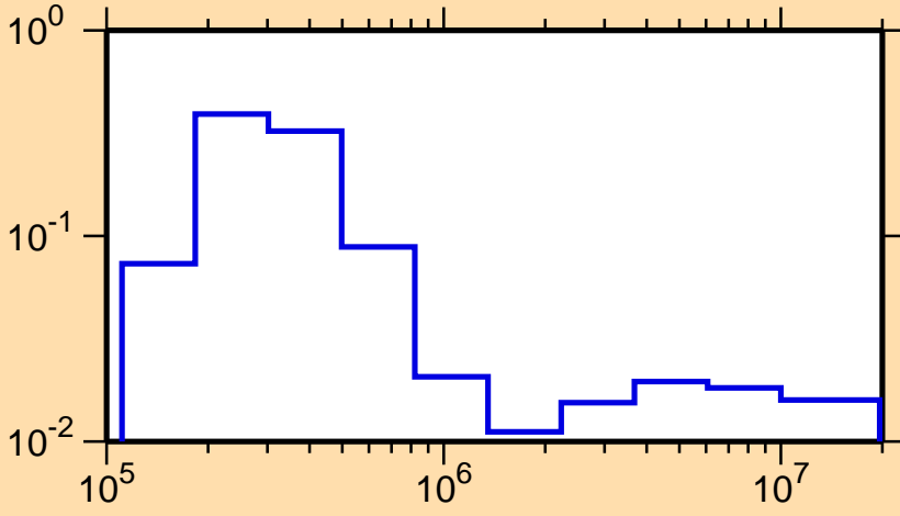
\sigma vs. E for ^{222}\text{Ac}(n,n_2)
