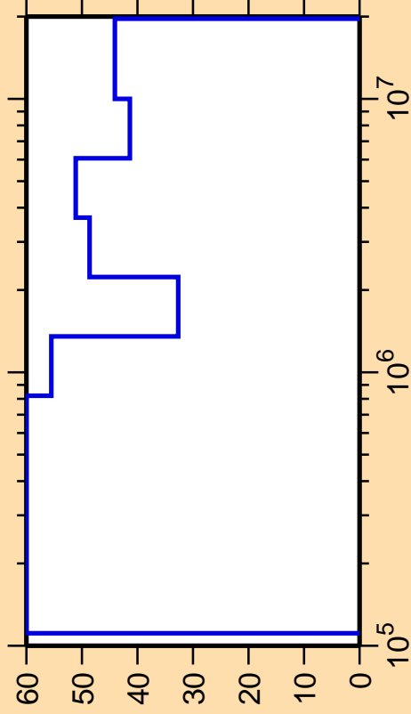
\Delta\sigma/\sigma vs. E for ^{222}\text{Ac}(n,n_2)
