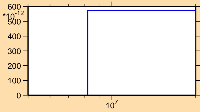
\sigma vs. E for ^{222}\text{Ac}(n,\text{He3})
