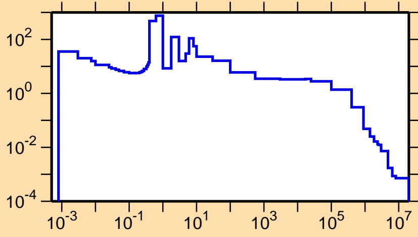
\sigma vs. E for ^{222}\text{Ac}(n,\gamma)
