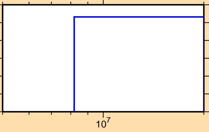
\sigma vs. E for ^{222}\text{Ac}(n,\text{nd})
