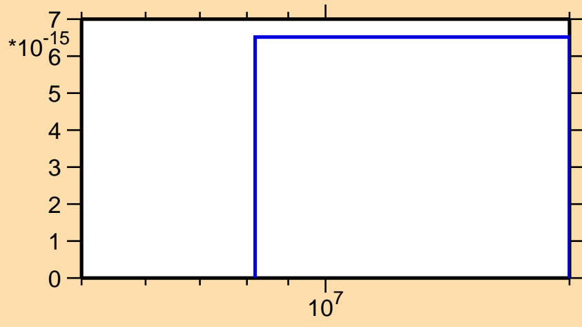
\sigma vs. E for ^{222}\text{Ac}(\text{mt } 42)
