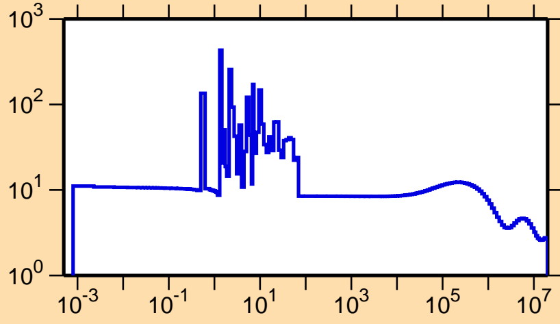
\sigma vs. E for ^{222}\text{Ac}(n,\text{el.})
