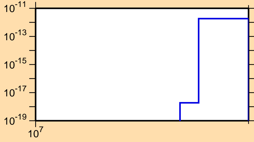
\sigma vs. E for ^{223}\text{Ac}(\text{mt } 42)
