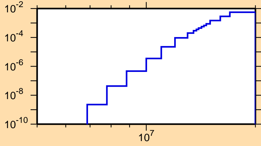
\sigma vs. E for ^{223}\text{Ac}(n,np)
