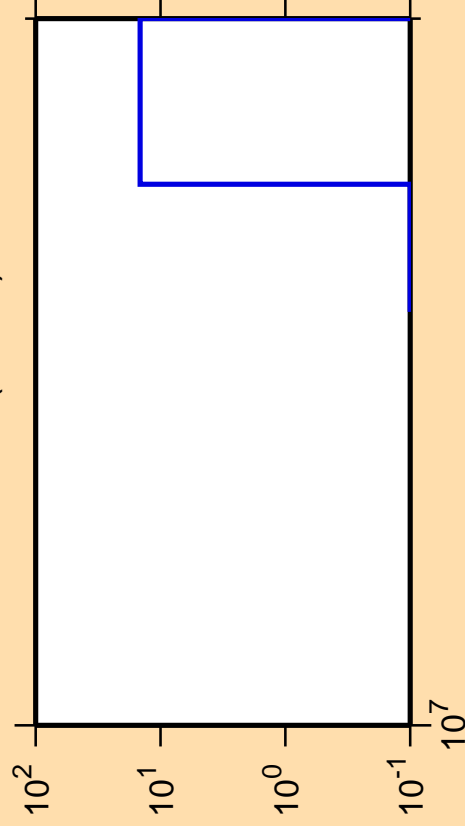
\Delta\sigma/\sigma vs. E for ^{223}\text{Ac}(\text{mt } 42)
