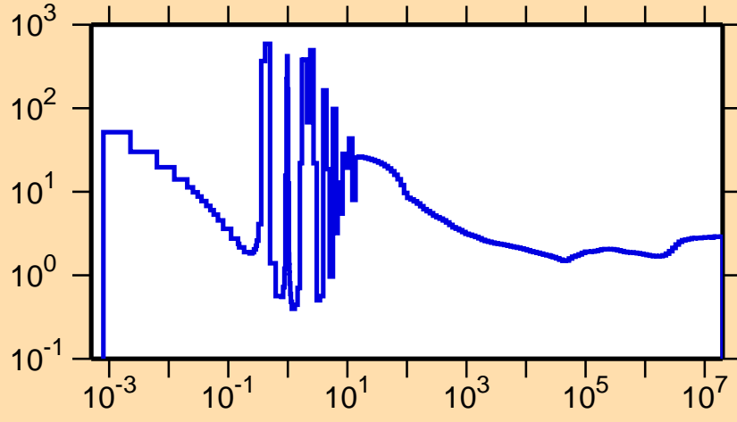
\sigma vs. E for ^{223}\text{Ac}(n,\text{nonel.})
