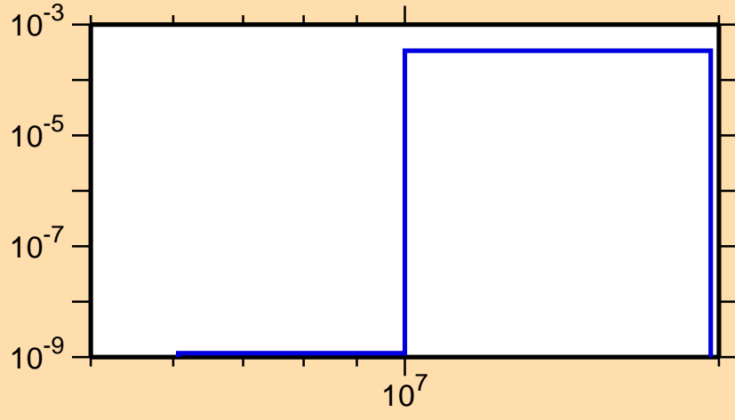
\sigma vs. E for ^{223}\text{Ac}(n,t)
