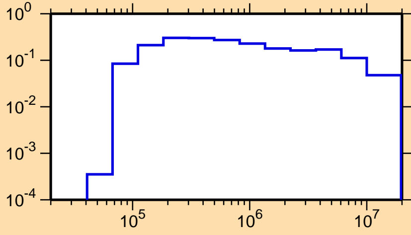
\sigma vs. E for ^{223}\text{Ac}(n,n_4)
