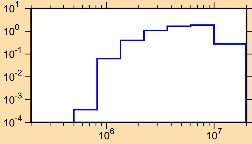
\sigma vs. E for ^{223}\text{Ac}(n,n\text{cont.})
