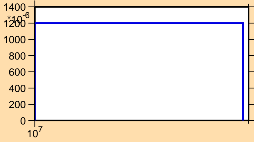
\sigma vs. E for ^{223}\text{Ac}(n,3n\alpha)
