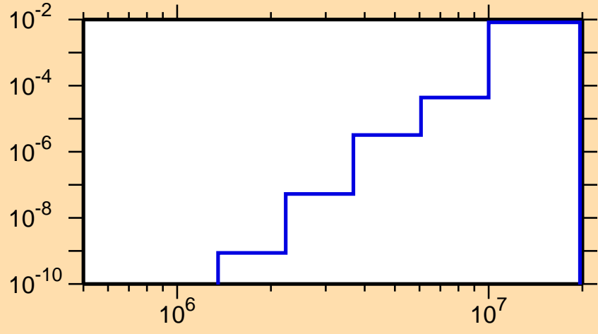
\sigma vs. E for ^{223}\text{Ac}(n,n\alpha)
