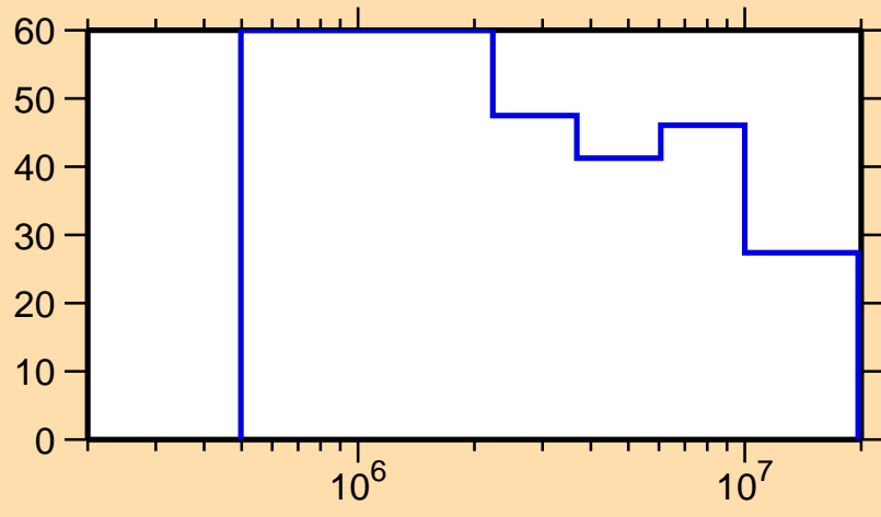
\Delta\sigma/\sigma vs. E for ^{223}\text{Ac}(n,n\text{cont.})
