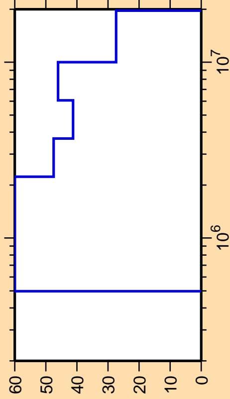
\Delta\sigma/\sigma vs. E for ^{223}\text{Ac}(n,n\text{cont.})
