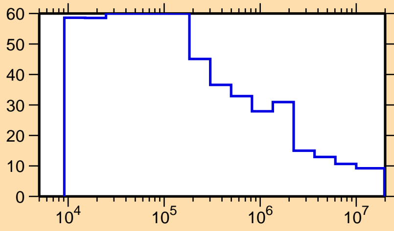
\Delta\sigma/\sigma vs. E for ^{223}\text{Ac}(n,\text{nonel.})
